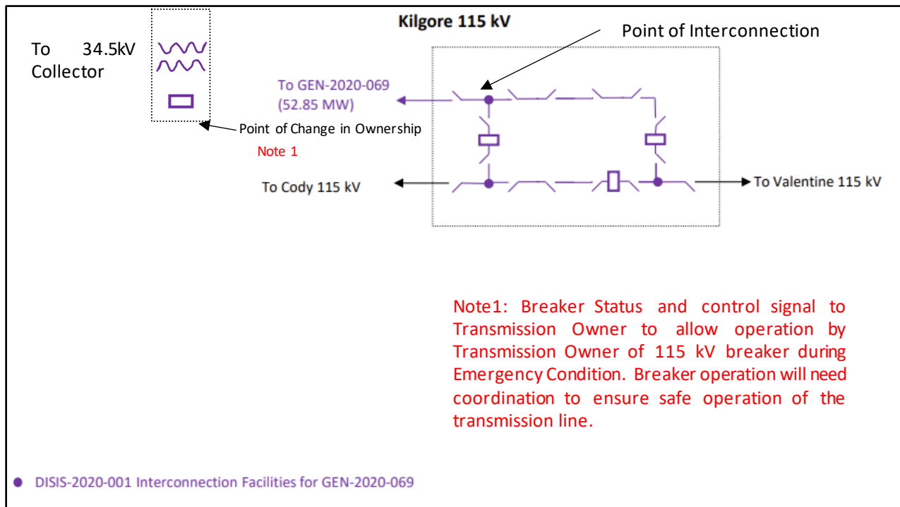
Figure A1: One-line Diagram of Point of Interconnection
